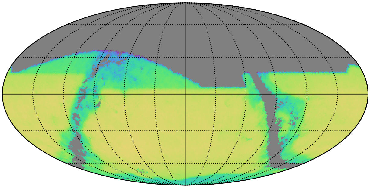
weather_cloudso20v3.4_10yrs z band and non-DD: QSONumberCountsMetric
