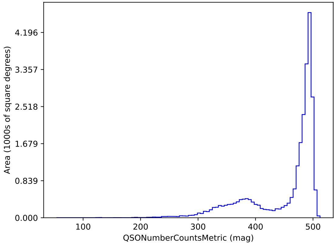
weather_cloudso20v3.4_10yrs z band and non-DD: QSONumberCountsMetric
