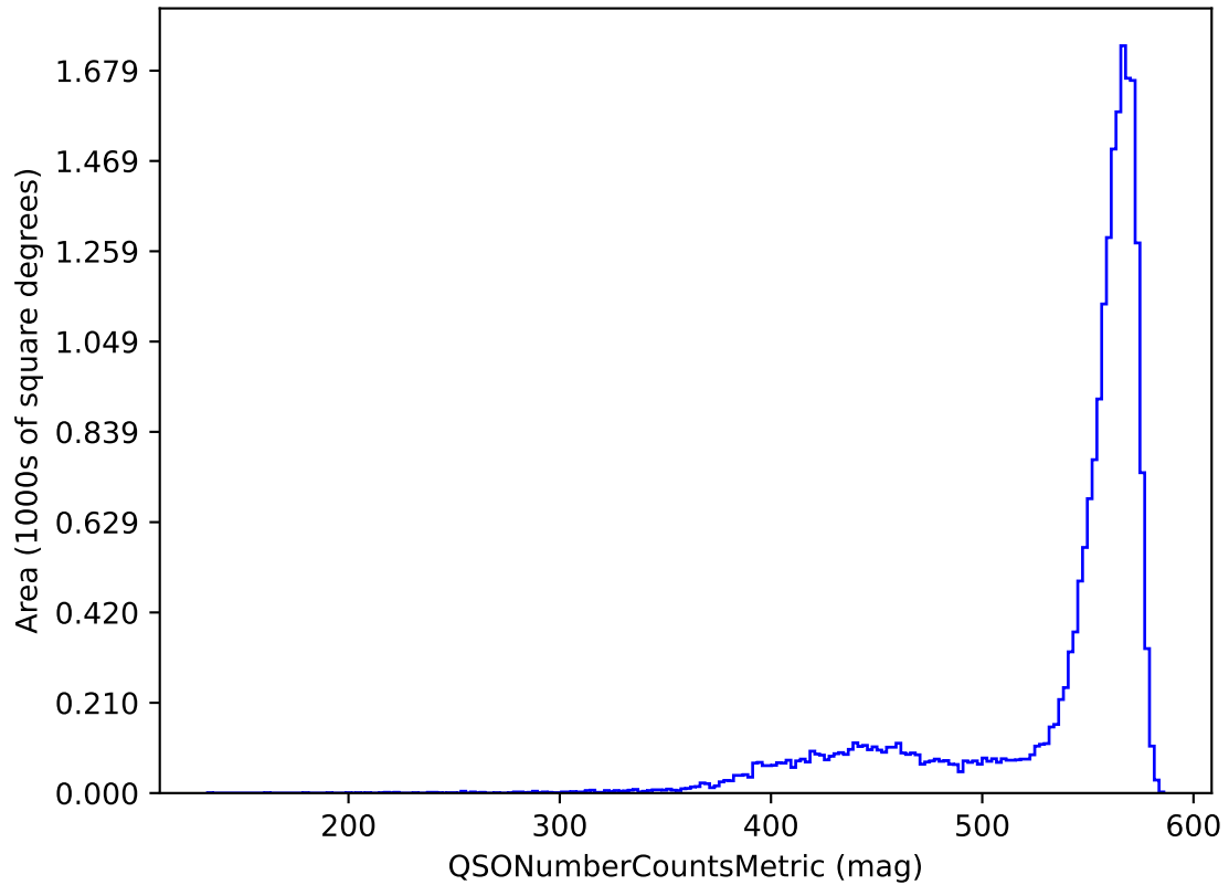
weather_cloudso20v3.4_10yrs y band and non-DD: QSONumberCountsMetric
