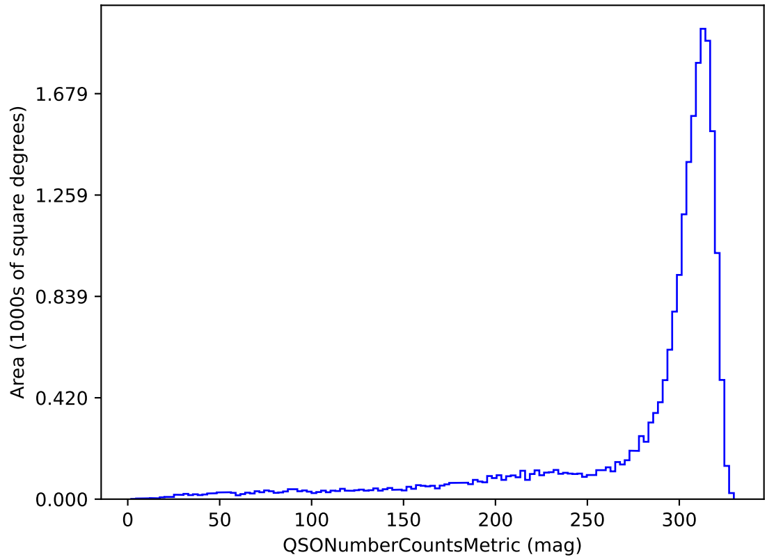
weather_cloudso20v3.4_10yrs u band and non-DD: QSONumberCountsMetric
