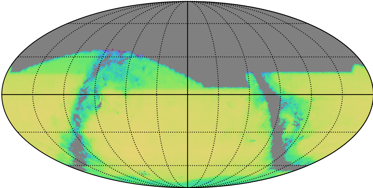
weather_cloudso20v3.4_10yrs r band and non-DD: QSONumberCountsMetric
