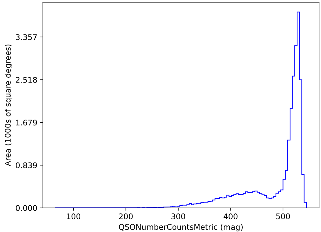
weather_cloudso20v3.4_10yrs r band and non-DD: QSONumberCountsMetric
