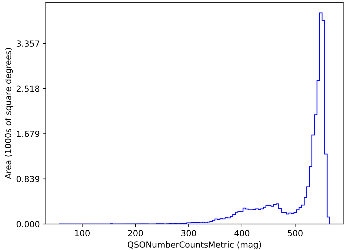
weather_cloudso20v3.4_10yrs i band and non-DD: QSONumberCountsMetric
