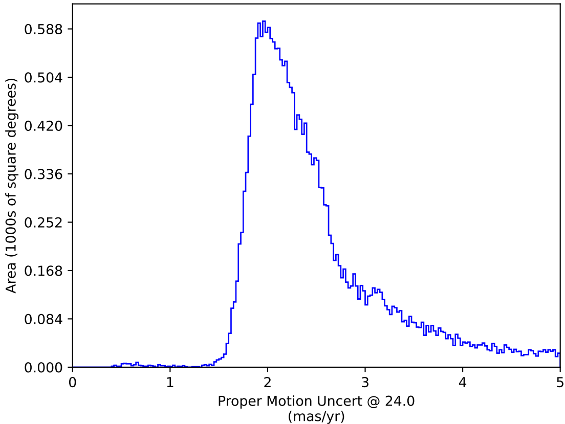
weather_cloudso20v3.4_10yrs : Proper Motion Uncert @ 24.0
