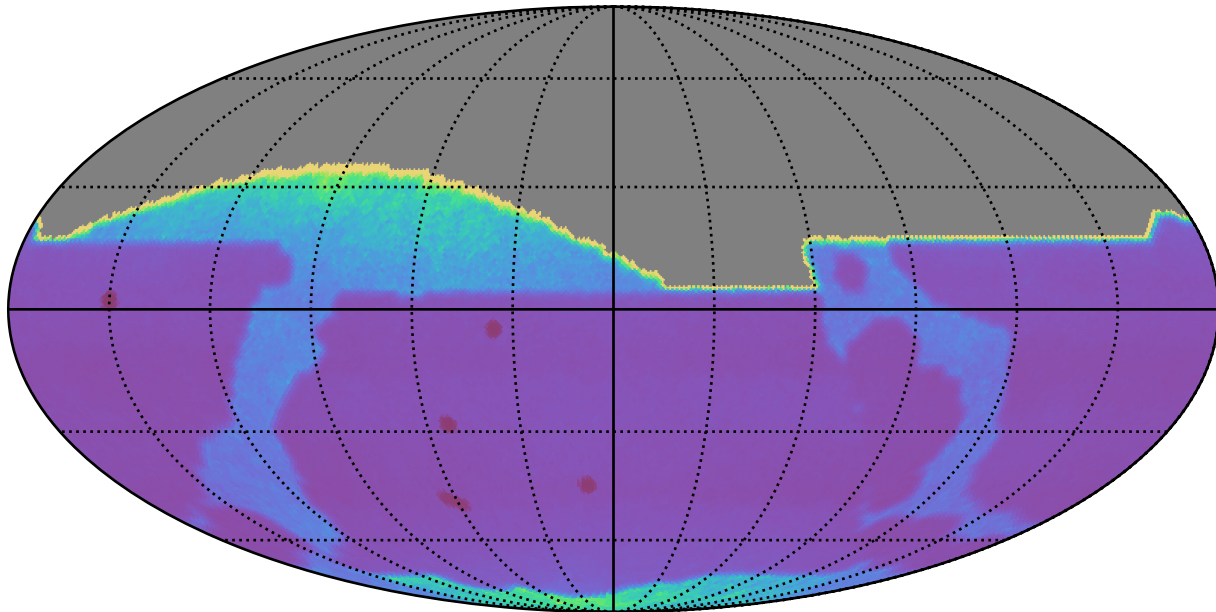
weather_cloudso20v3.4_10yrs : Proper Motion Uncert @ 20.5
