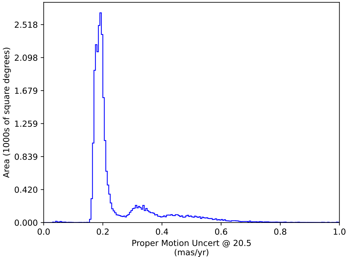
weather_cloudso20v3.4_10yrs : Proper Motion Uncert @ 20.5
