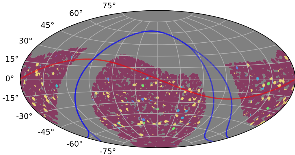
weather_cloudso20v3.4_10yrs : PrestoKNe_score_p
