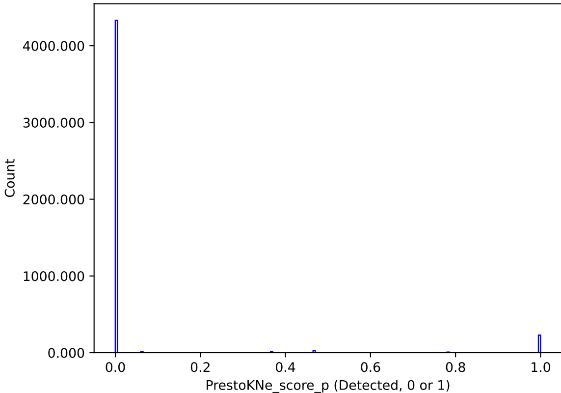
weather_cloudso20v3.4_10yrs : PrestoKNe_score_p
