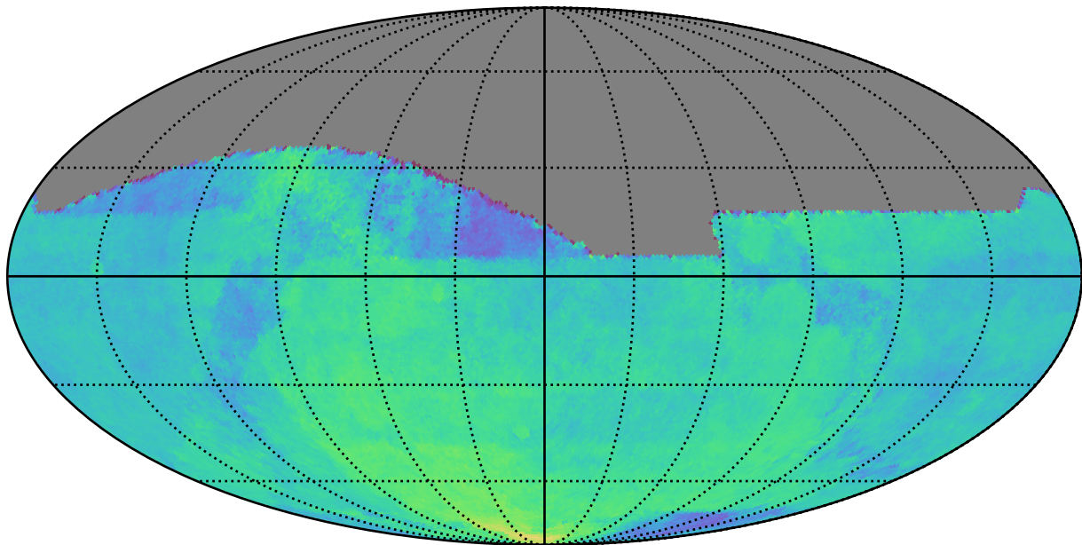
weather_cloudso20v3.4_10yrs : Parallax Coverage @ 24.0
