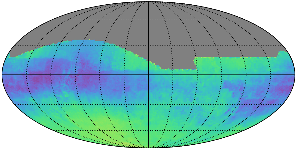
weather_cloudso20v3.4_10yrs : Parallax-DCR degeneracy @ 24.0
