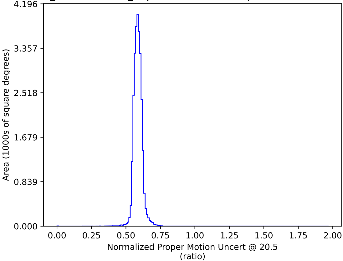
weather_cloudso20v3.4_10yrs : Normalized Proper Motion Uncert @ 20.5
