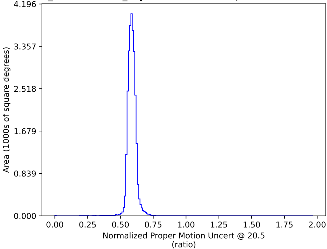
weather_cloudso20v3.4_10yrs : Normalized Proper Motion Uncert @ 20.5
