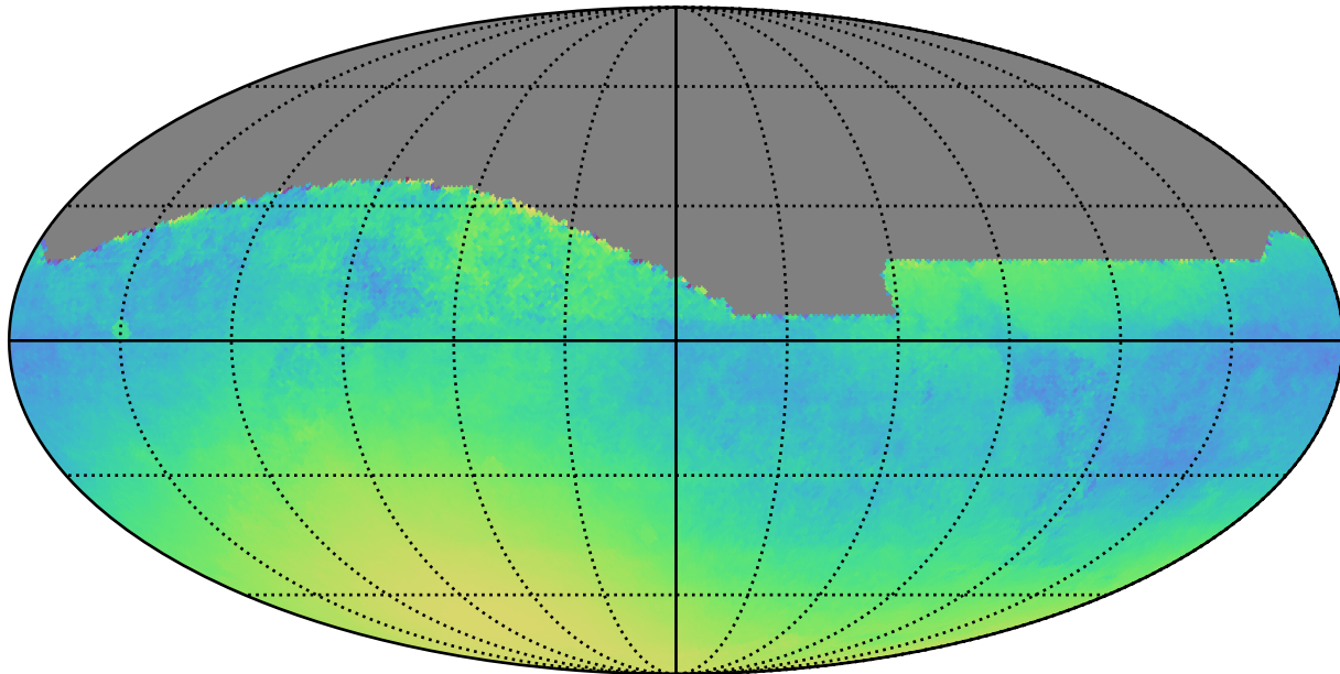
weather_cloudso20v3.4_10yrs : Normalized Parallax Uncert @ 24.0
