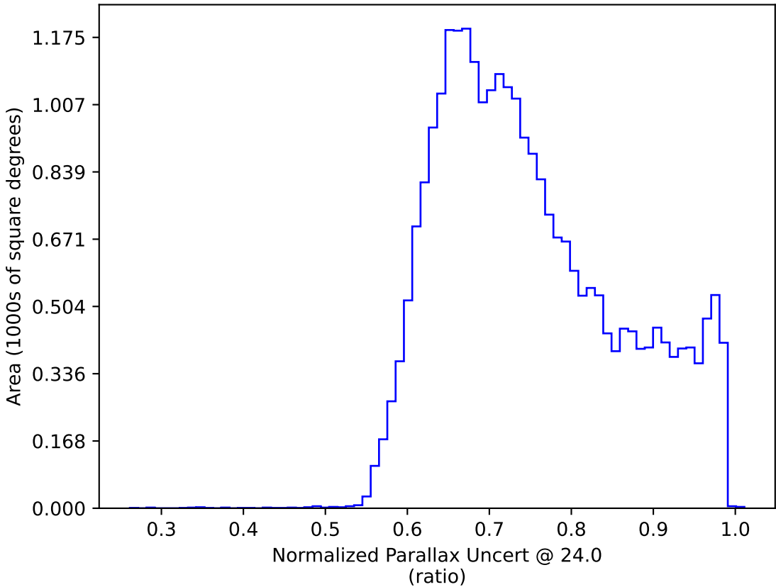
weather_cloudso20v3.4_10yrs : Normalized Parallax Uncert @ 24.0
