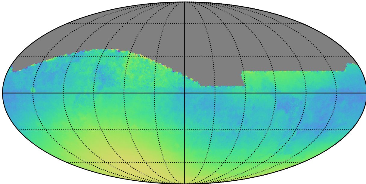
weather_cloudso20v3.4_10yrs : Normalized Parallax Uncert @ 22.4
