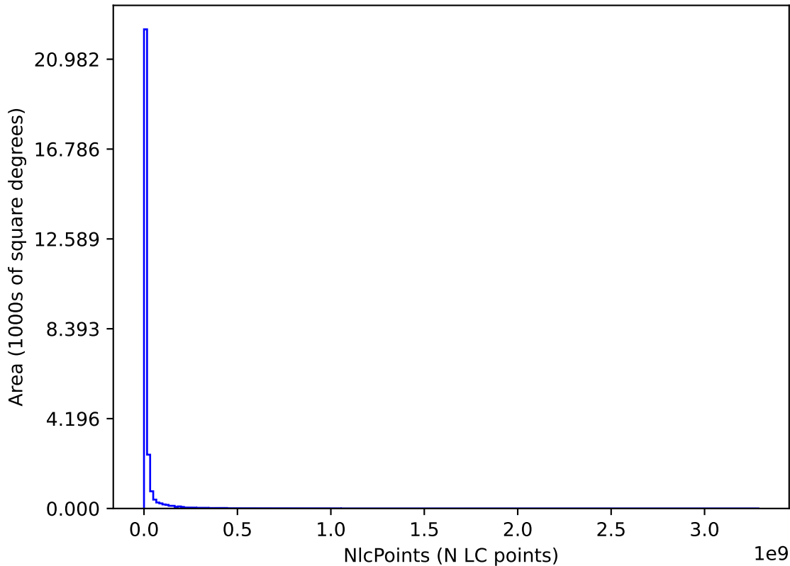
weather_cloudso20v3.4_10yrs : NlcPoints
