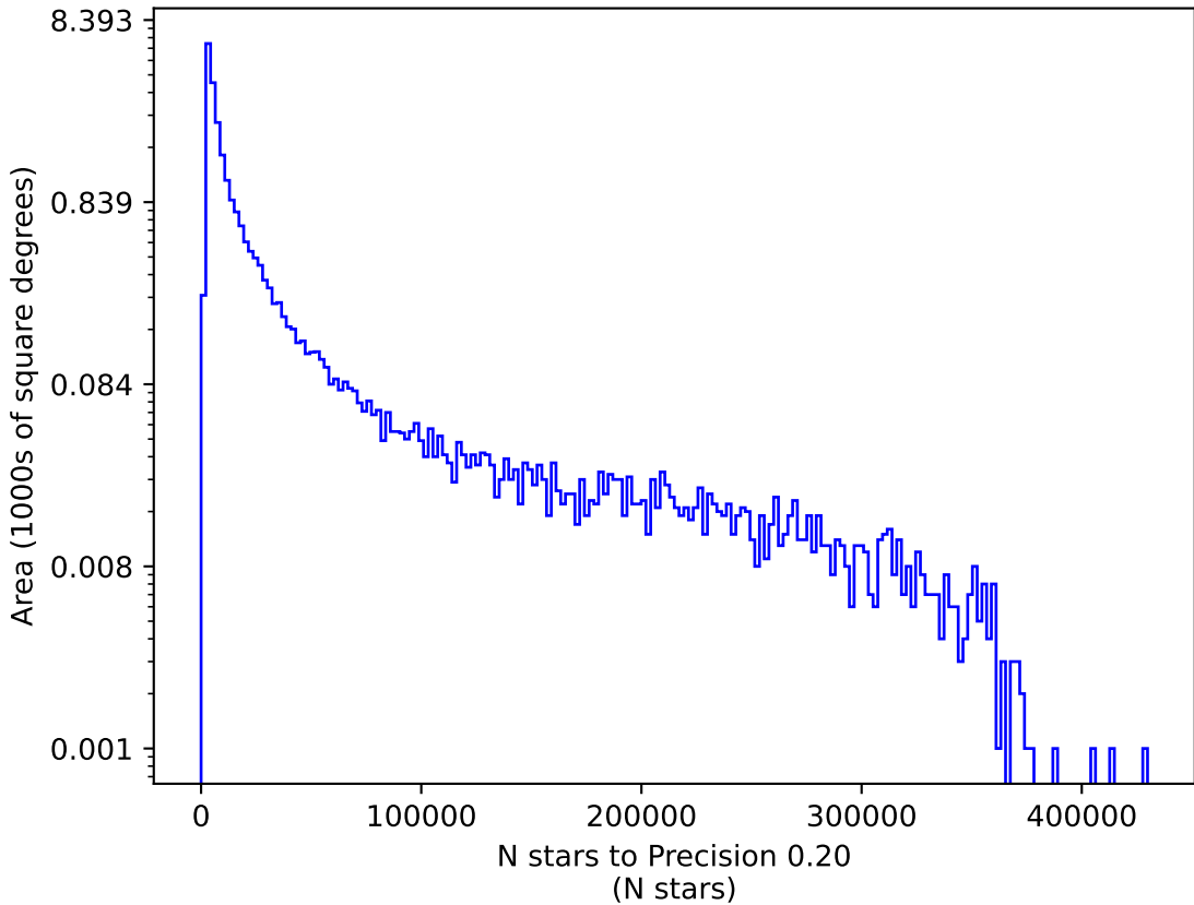
weather_cloudso20v3.4_10yrs u: N stars to Precision 0.20
