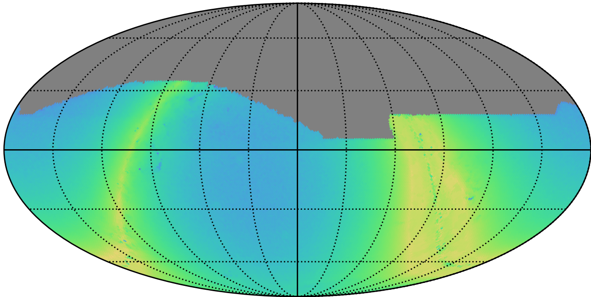
weather_cloudso20v3.4_10yrs r: N stars to Precision 0.20
