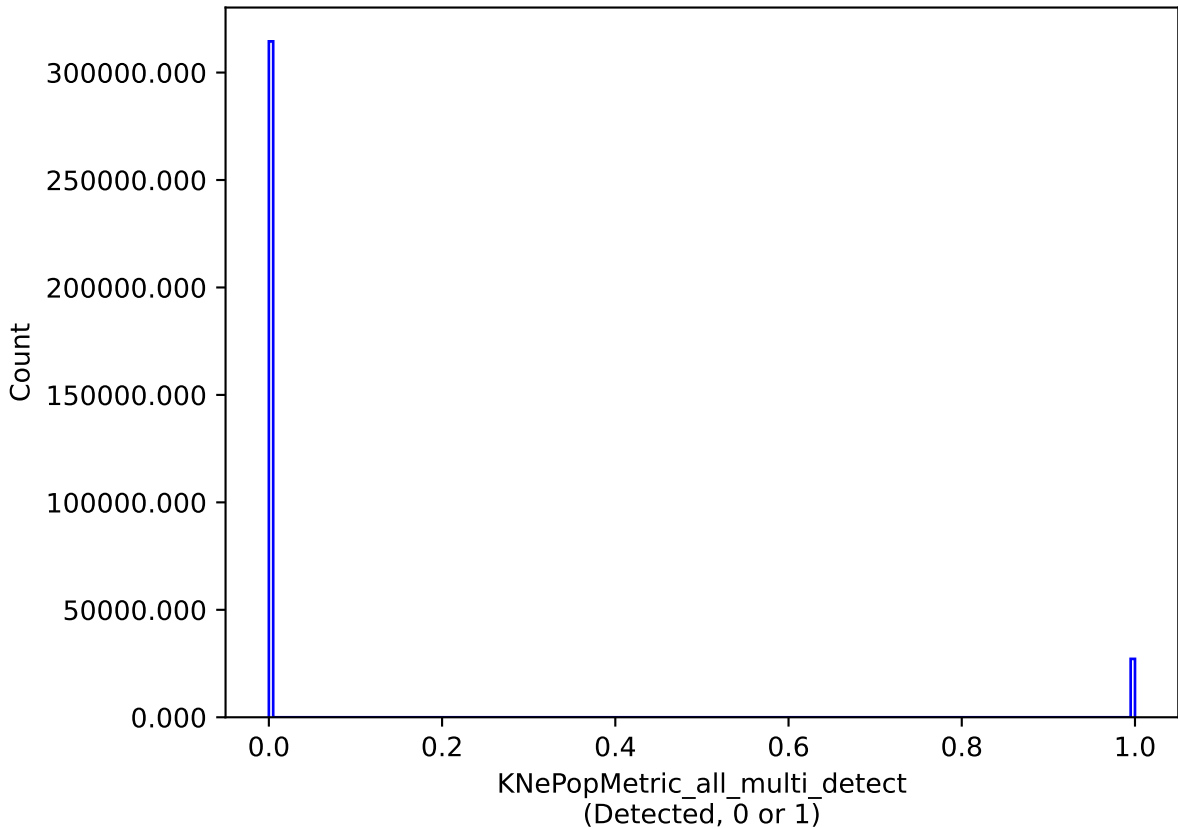
weather_cloudso20v3.4_10yrs all models: KNePopMetric_all_multi_detect
