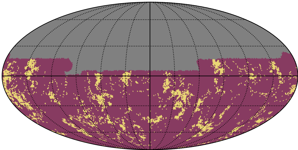
weather_cloudso20v3.4_10yrs u band: Gaps_3hr
