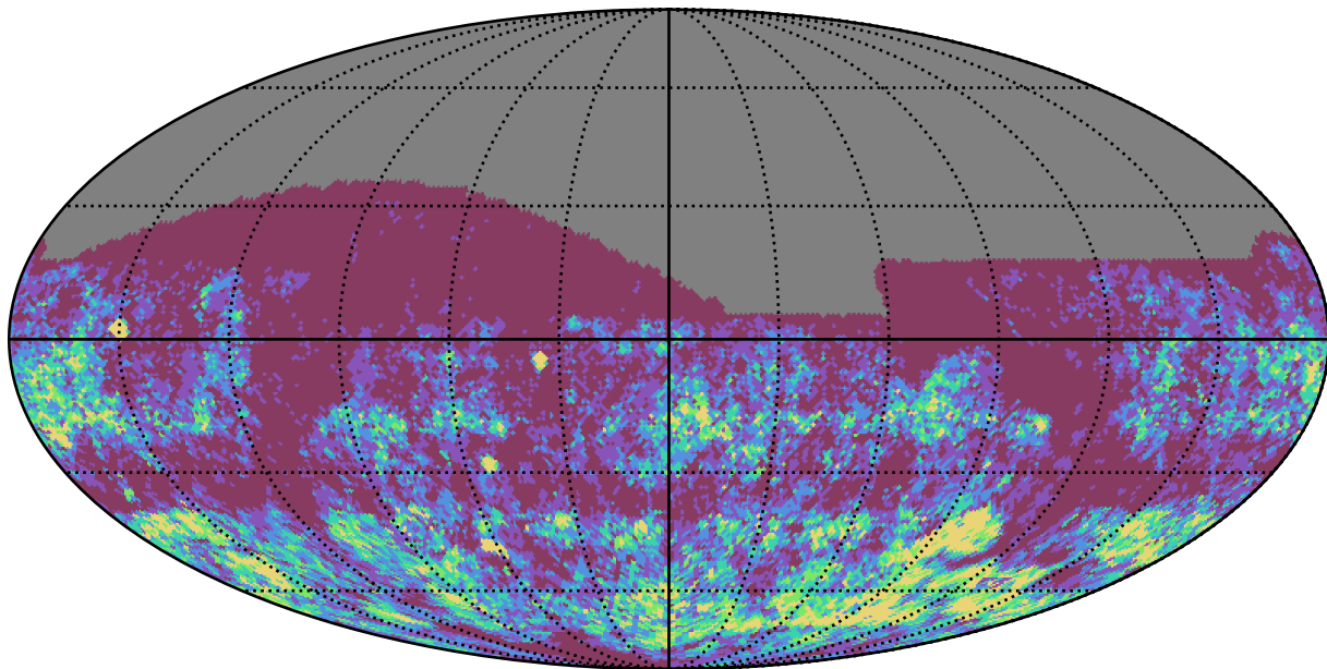
weather_cloudso20v3.4_10yrs r band: Gaps_3hr
