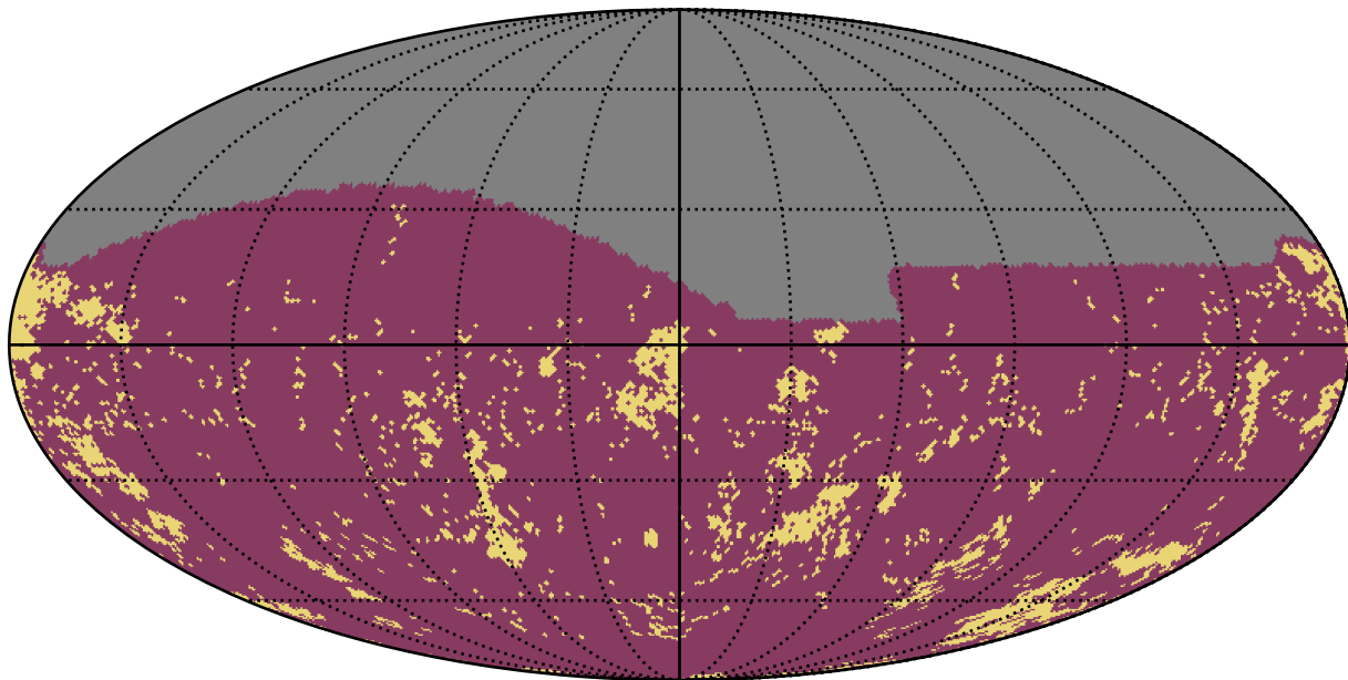
weather_cloudso20v3.4_10yrs g band: Gaps_3hr
