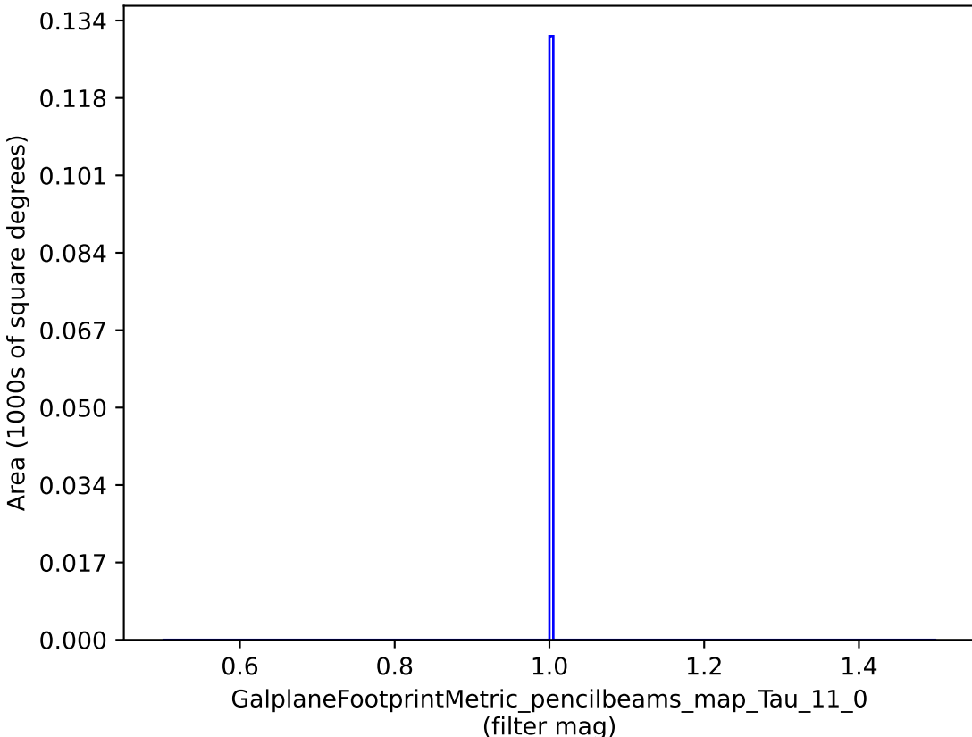
weather_cloudso20v3.4_10yrs : GalplaneFootprintMetric_pencilbeams_map_Tau_11_0
