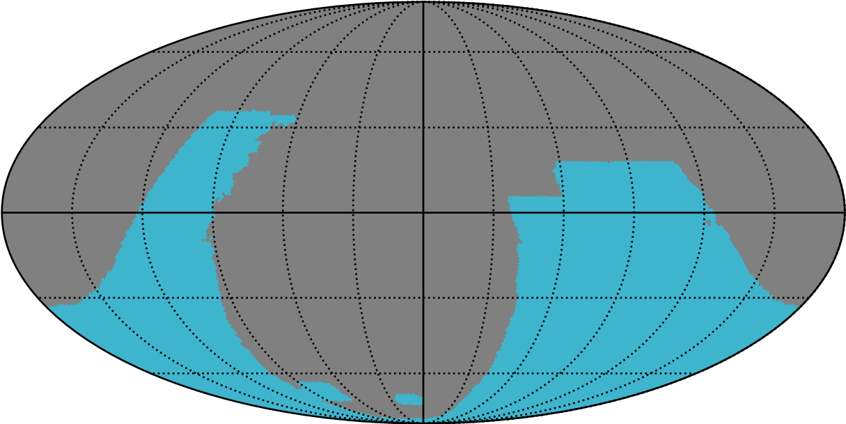
weather_cloudso20v3.4_10yrs : GalplaneFootprintMetric_galactic_plane_map_Tau_2_0
