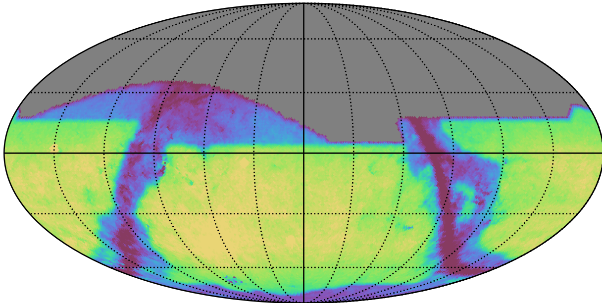
weather_cloudso20v3.4_10yrs z: GalaxyCountsMetricExtended
