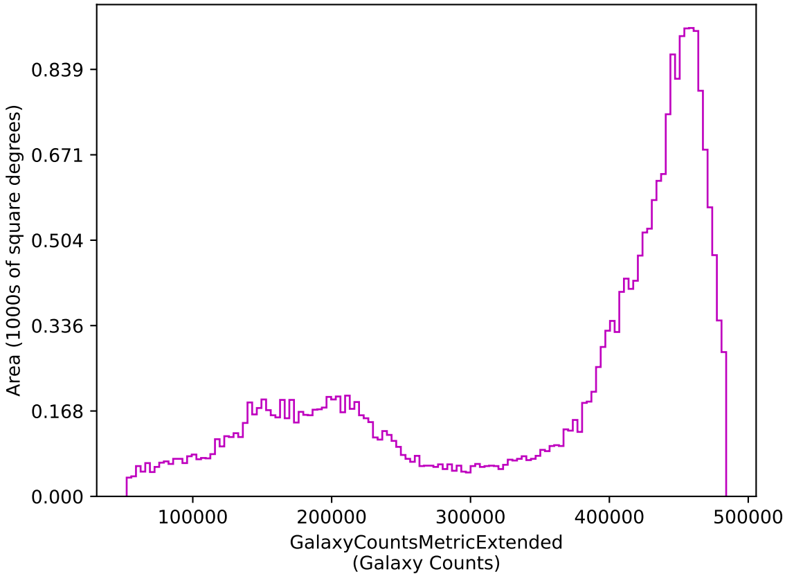
weather_cloudso20v3.4_10yrs z: GalaxyCountsMetricExtended
