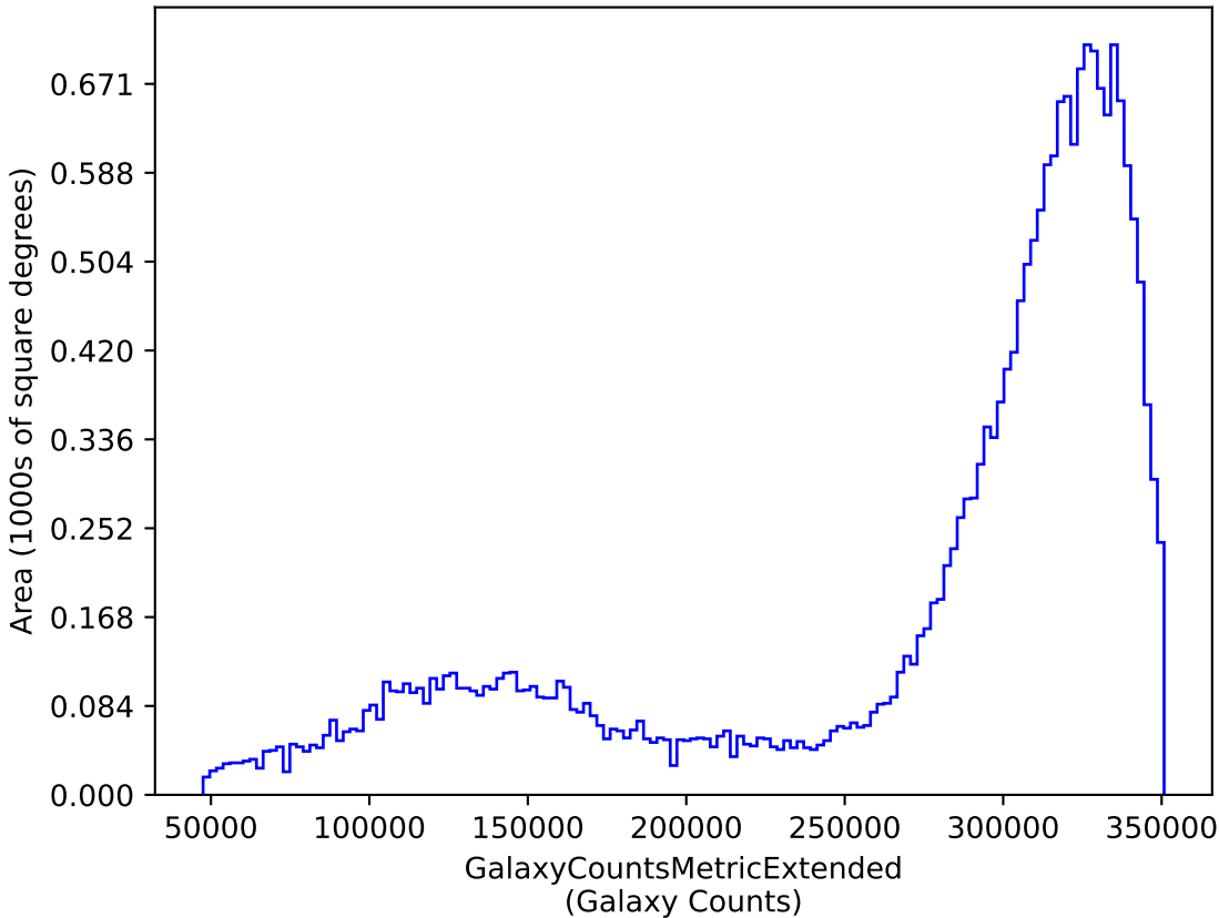
weather_cloudso20v3.4_10yrs y: GalaxyCountsMetricExtended
