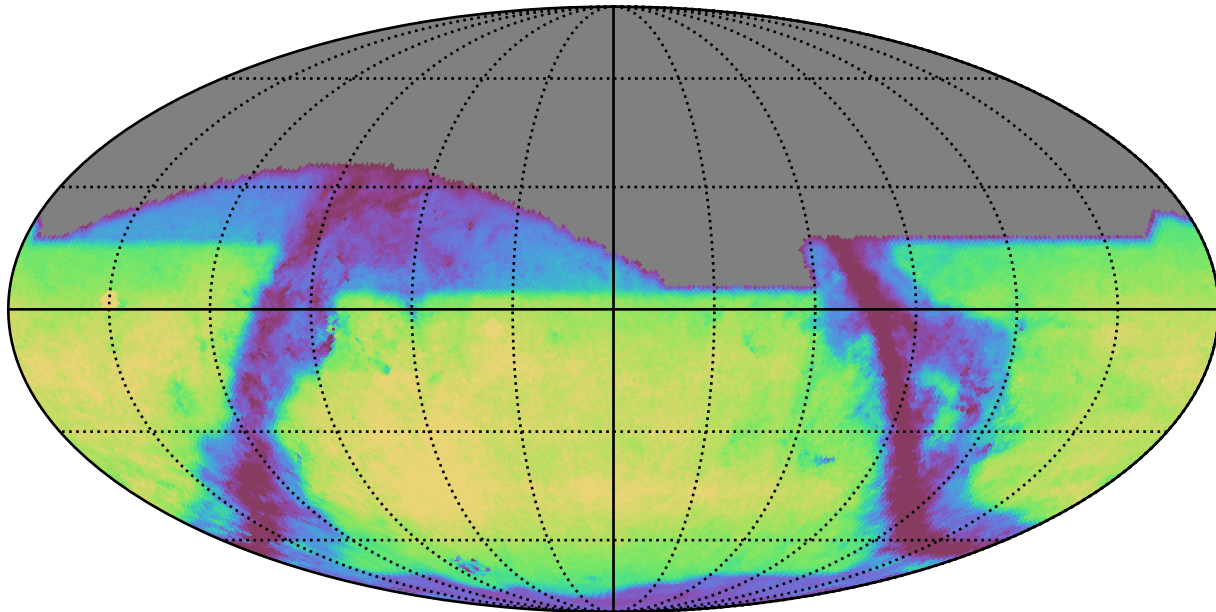
weather_cloudso20v3.4_10yrs i: GalaxyCountsMetricExtended
