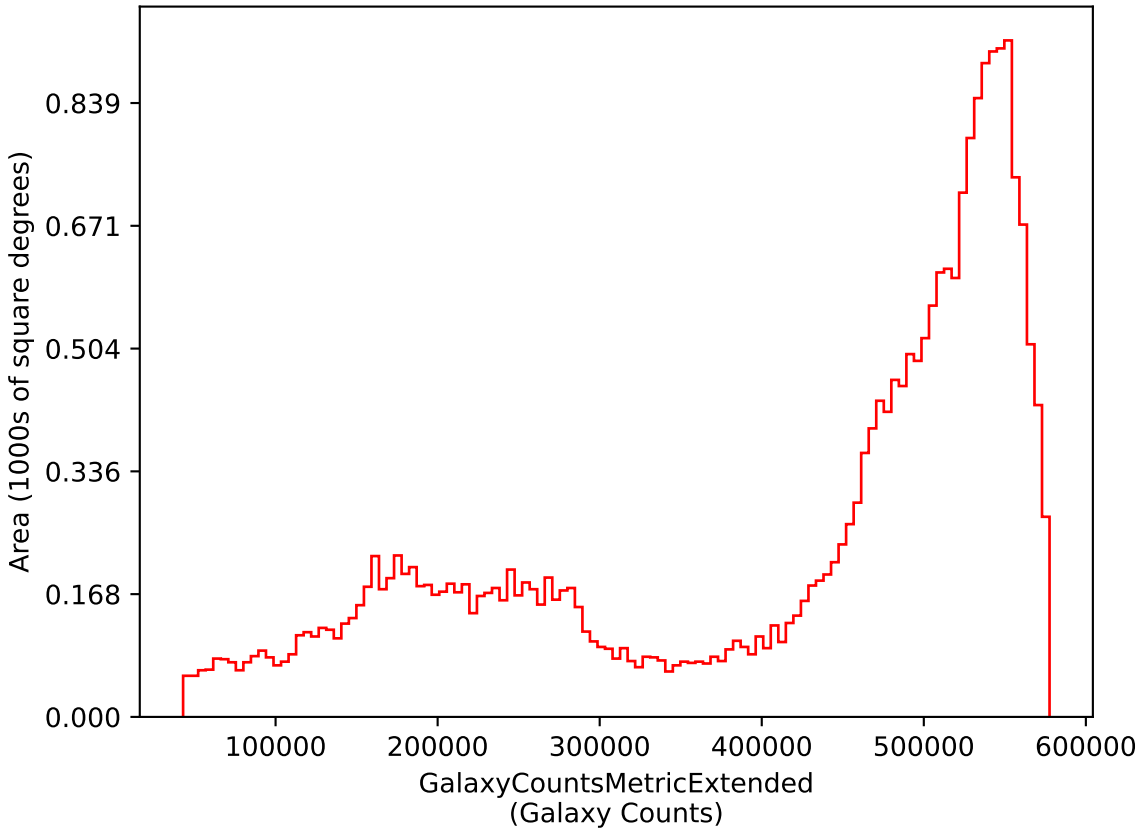
weather_cloudso20v3.4_10yrs i: GalaxyCountsMetricExtended
