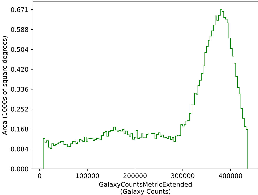
weather_cloudso20v3.4_10yrs g: GalaxyCountsMetricExtended
