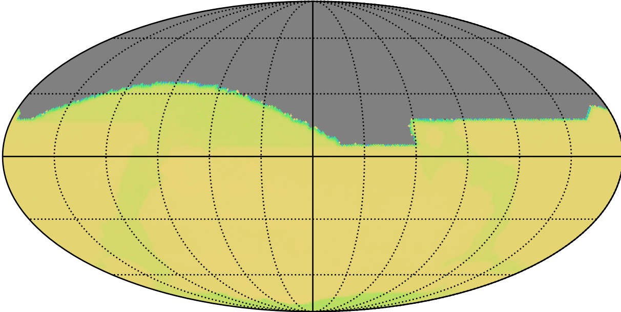
weather_cloudso20v3.4_10yrs : GalPlaneVisitIntervalsTimescales_xray_binaries_map_Tau_73_0
