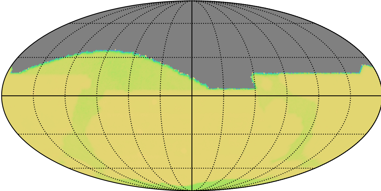
weather_cloudso20v3.4_10yrs : GalPlaneVisitIntervalsTimescales_xray_binaries_map_Tau_46_5
