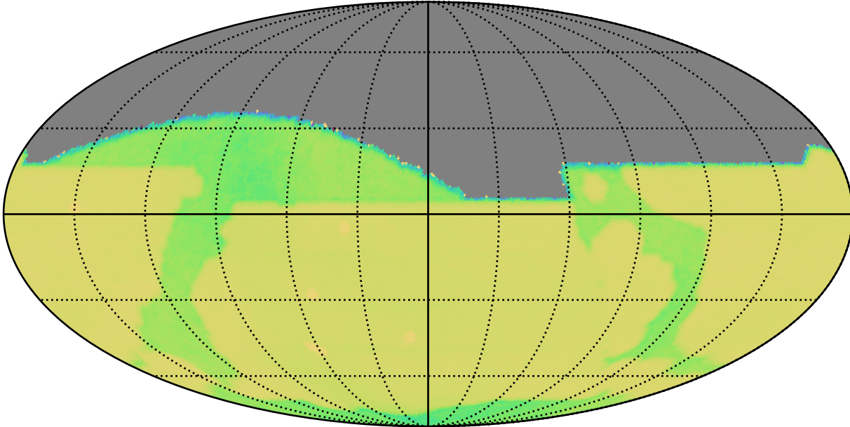
weather_cloudso20v3.4_10yrs : GalPlaneVisitIntervalsTimescales_xray_binaries_map_Tau_11_0
