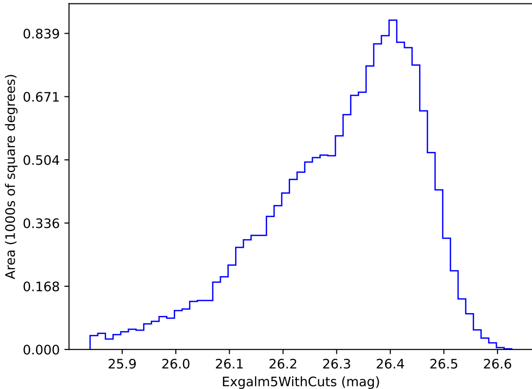
weather_cloudso20v3.4_10yrs i band non-DD year 9: ExgalM5WithCuts
