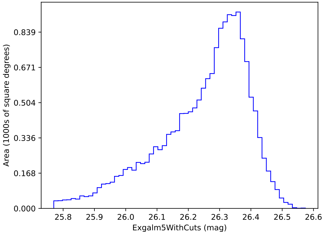
weather_cloudso20v3.4_10yrs i band non-DD year 8: ExgalM5WithCuts
