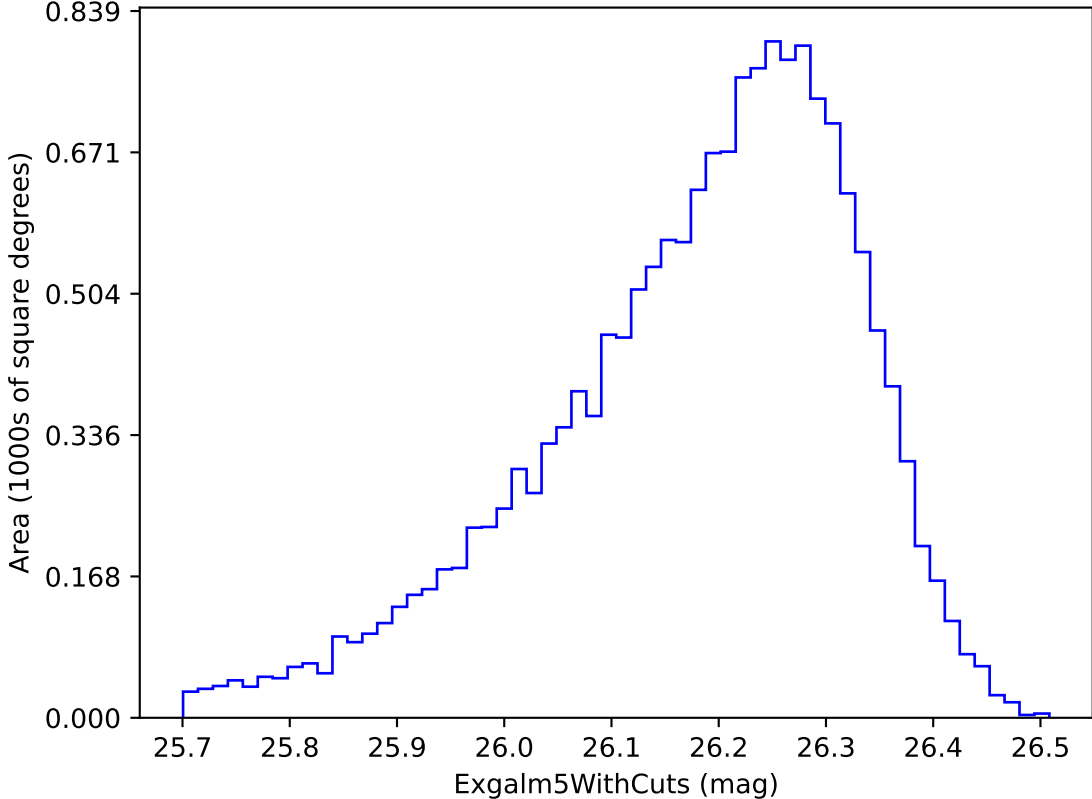
weather_cloudso20v3.4_10yrs i band non-DD year 7: ExgalM5WithCuts
