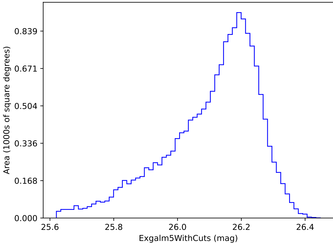
weather_cloudso20v3.4_10yrs i band non-DD year 6: ExgalM5WithCuts
