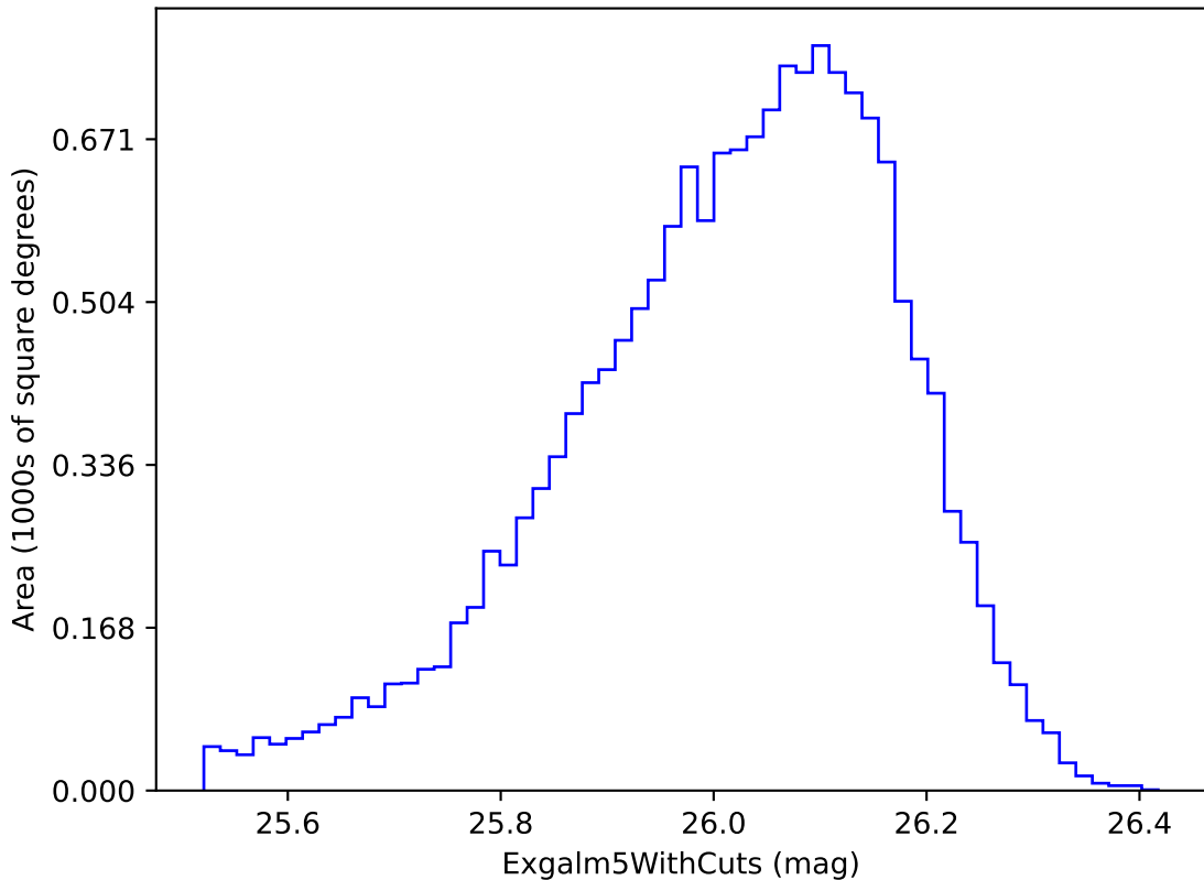
weather_cloudso20v3.4_10yrs i band non-DD year 5: ExgalM5WithCuts
