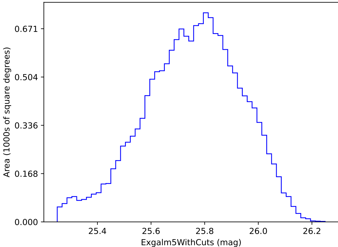
weather_cloudso20v3.4_10yrs i band non-DD year 3: Exgalml5WithCuts
