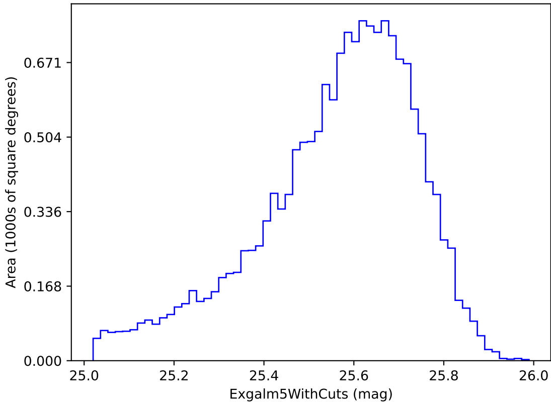
weather_cloudso20v3.4_10yrs i band non-DD year 2: ExgalM5WithCuts
