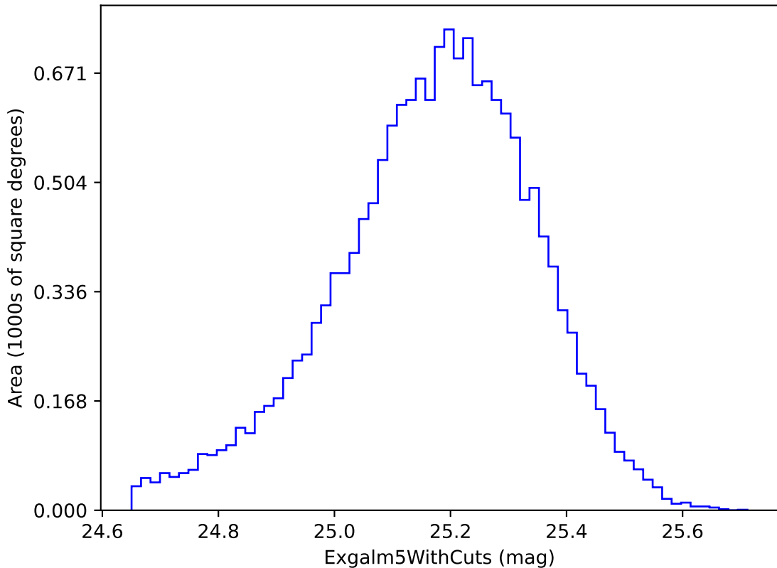
weather_cloudso20v3.4_10yrs i band non-DD year 1: ExgalM5WithCuts
