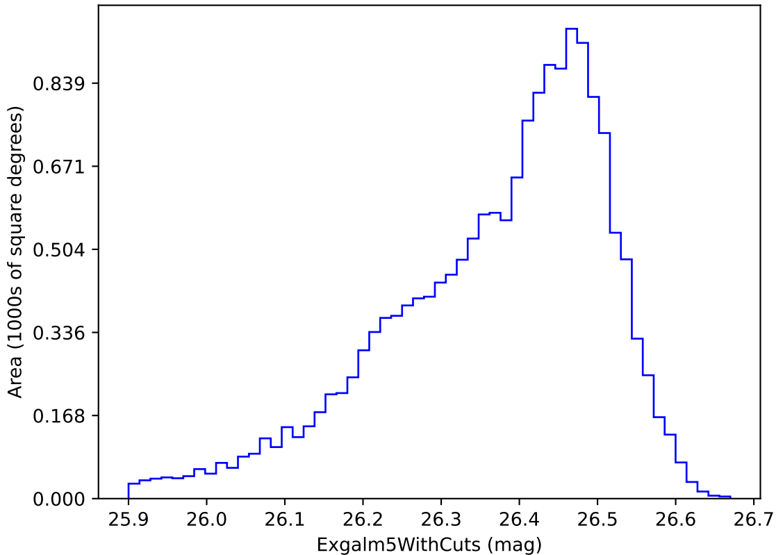
weather_cloudso20v3.4_10yrs i band non-DD year 10: Exgalml5WithCuts
