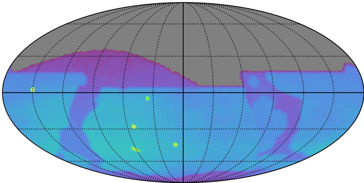
weather_cloudso20v3.4_10yrs : Brown Dwarf, L7
