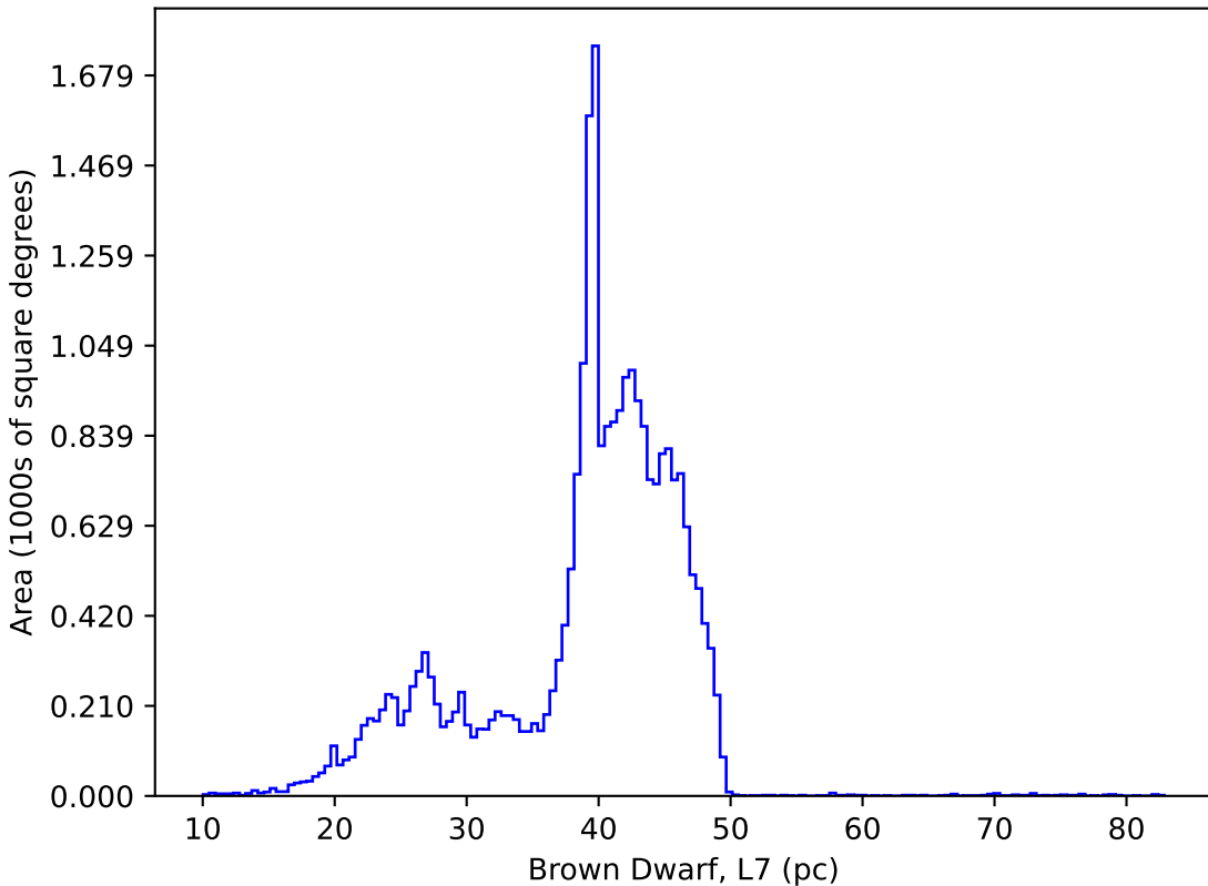
weather_cloudso20v3.4_10yrs : Brown Dwarf, L7
