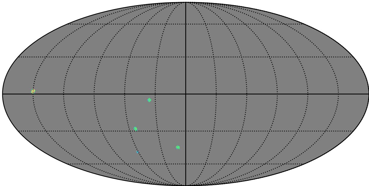
weather_cloudso20v3.4_10yrs z band: AGN_TimeLag_5_days
