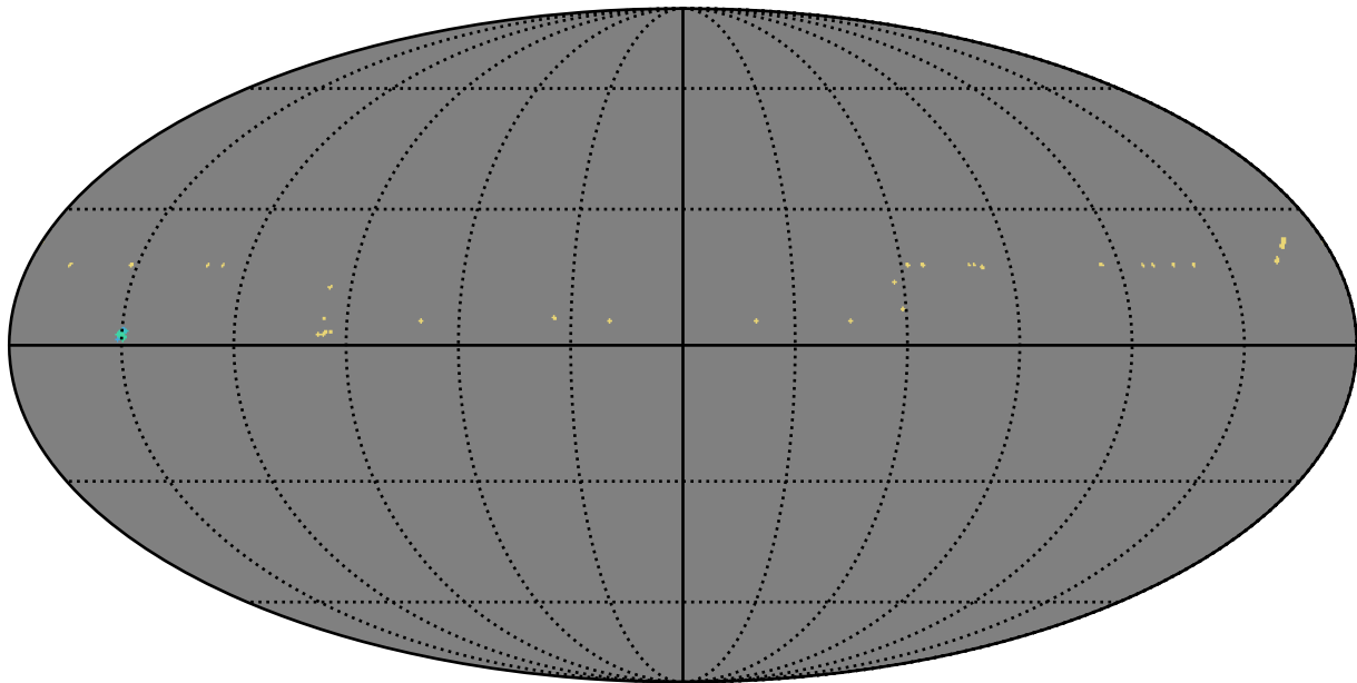
weather_cloudso20v3.4_10yrs y band: AGN_TimeLag_5_days
