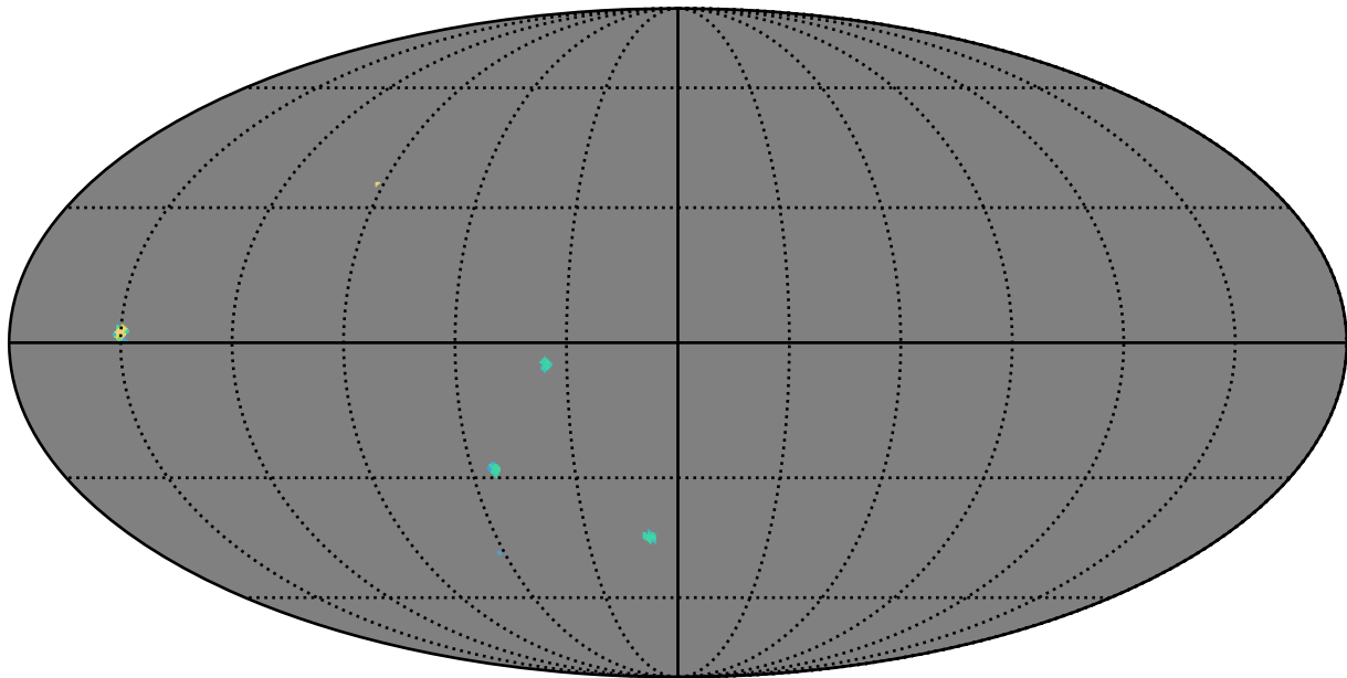
weather_cloudso20v3.4_10yrs r band: AGN_TimeLag_5_days
